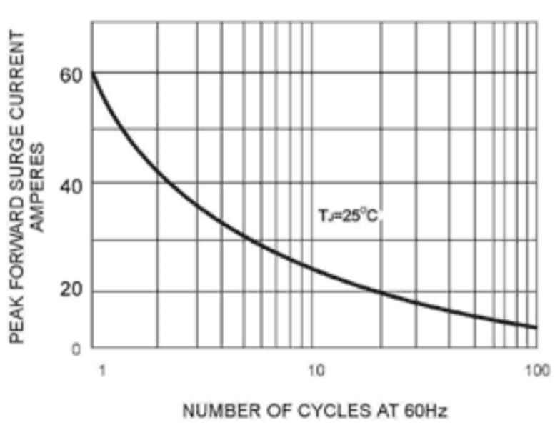
FIG. 4 - MAXIMUM FORWARD SURGE CURRENT
