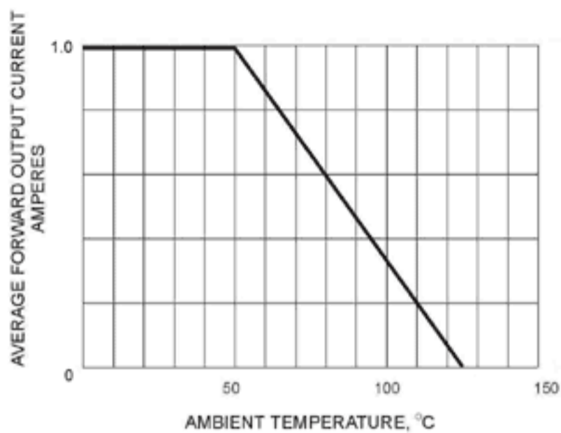
FIG. 1 - DERATING CURVE OUTPUT RECTIFIED CURRENT
